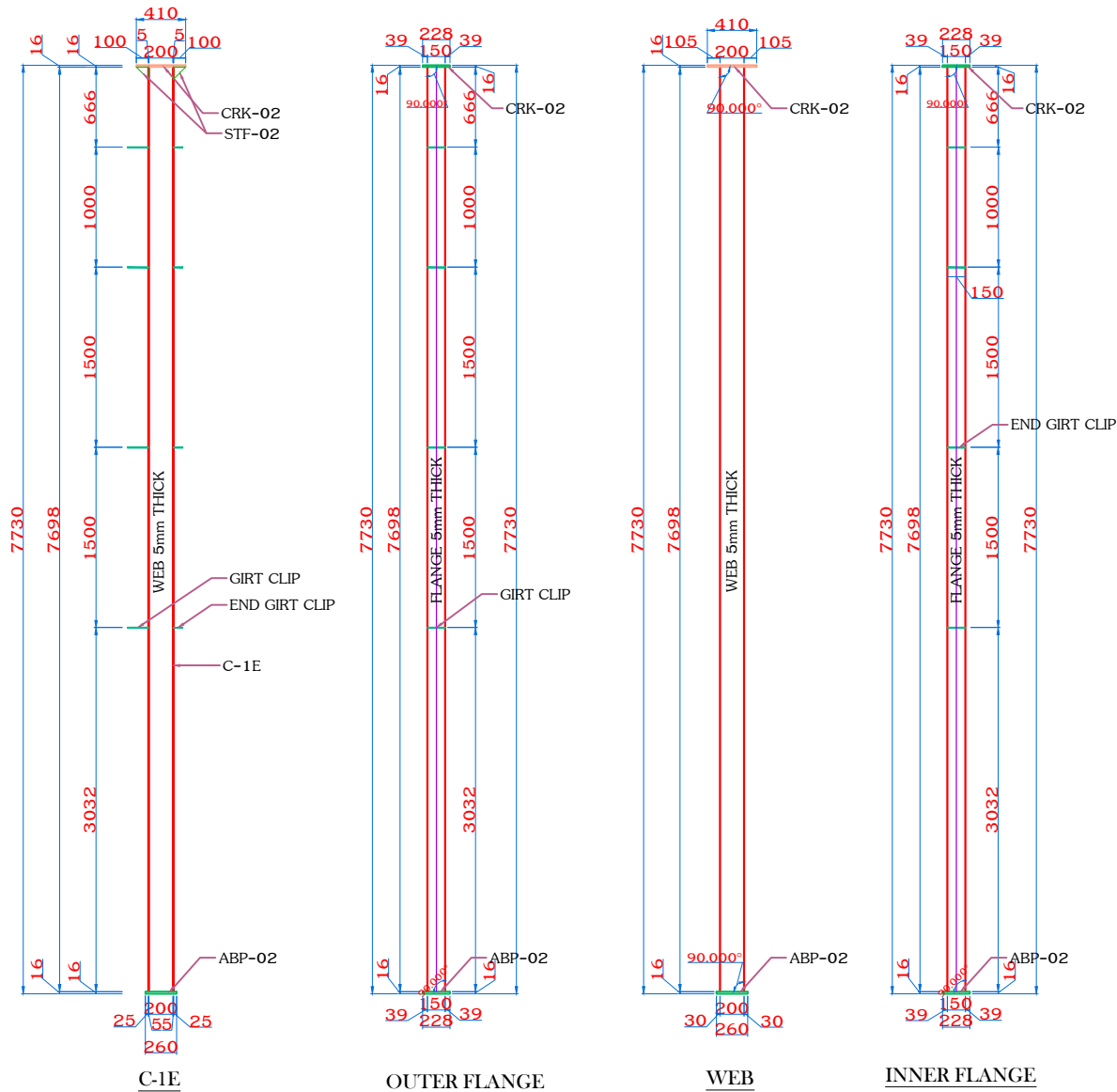
COLUMN DETAIL C-1E @ GRID 1 & 5 QTY:(02,L)(02,R)
